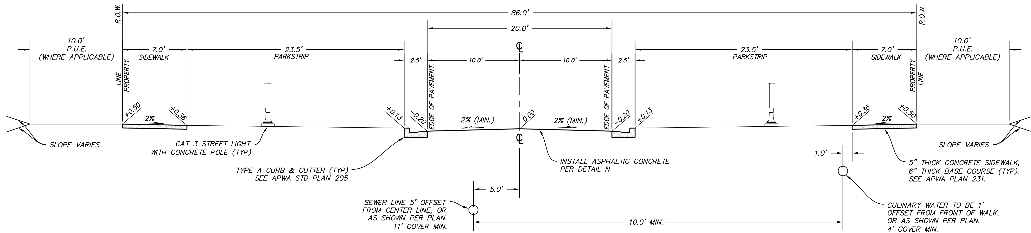
CONNECTOR BUMP OUT - 86' ROW CROSSWATER ROAD
