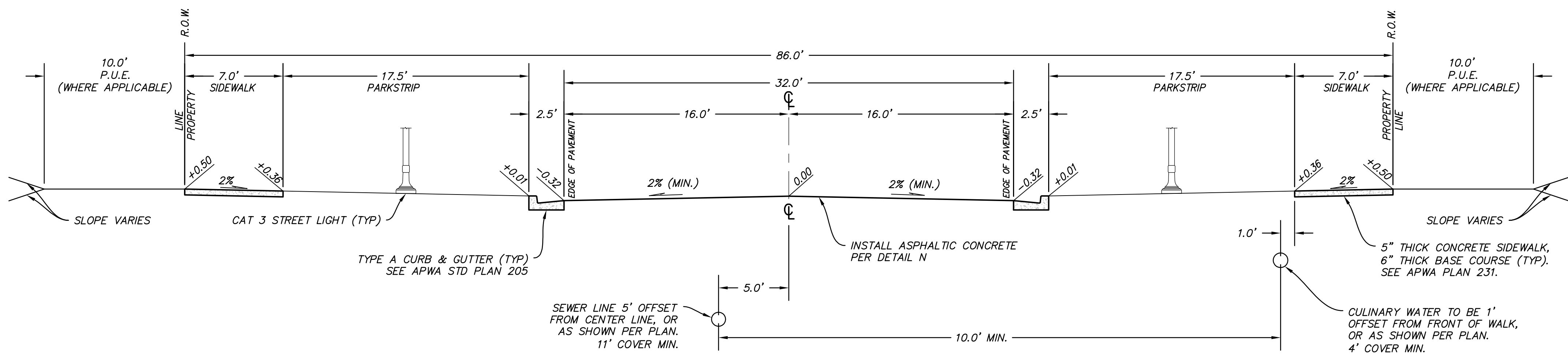
CONNECTOR - 86' ROW CROSSWATER ROAD
