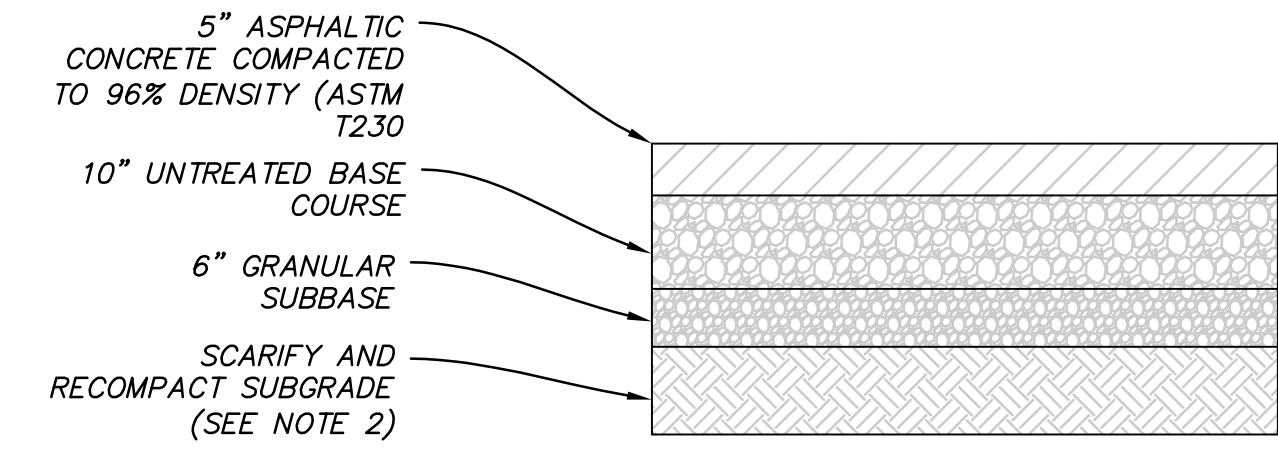
PAVEMENT SECTION (COLLECTOR & CONNECTOR)
